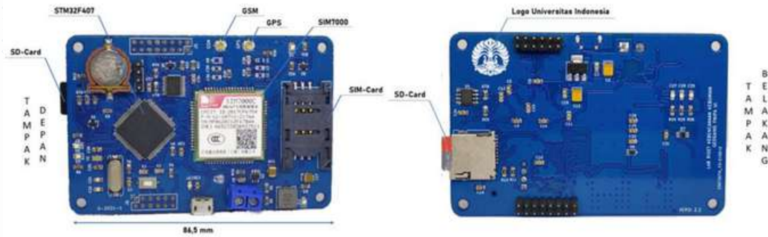
Gambar 3.11 Modul Mikrokontroler eDUcation, Research and developmENT
